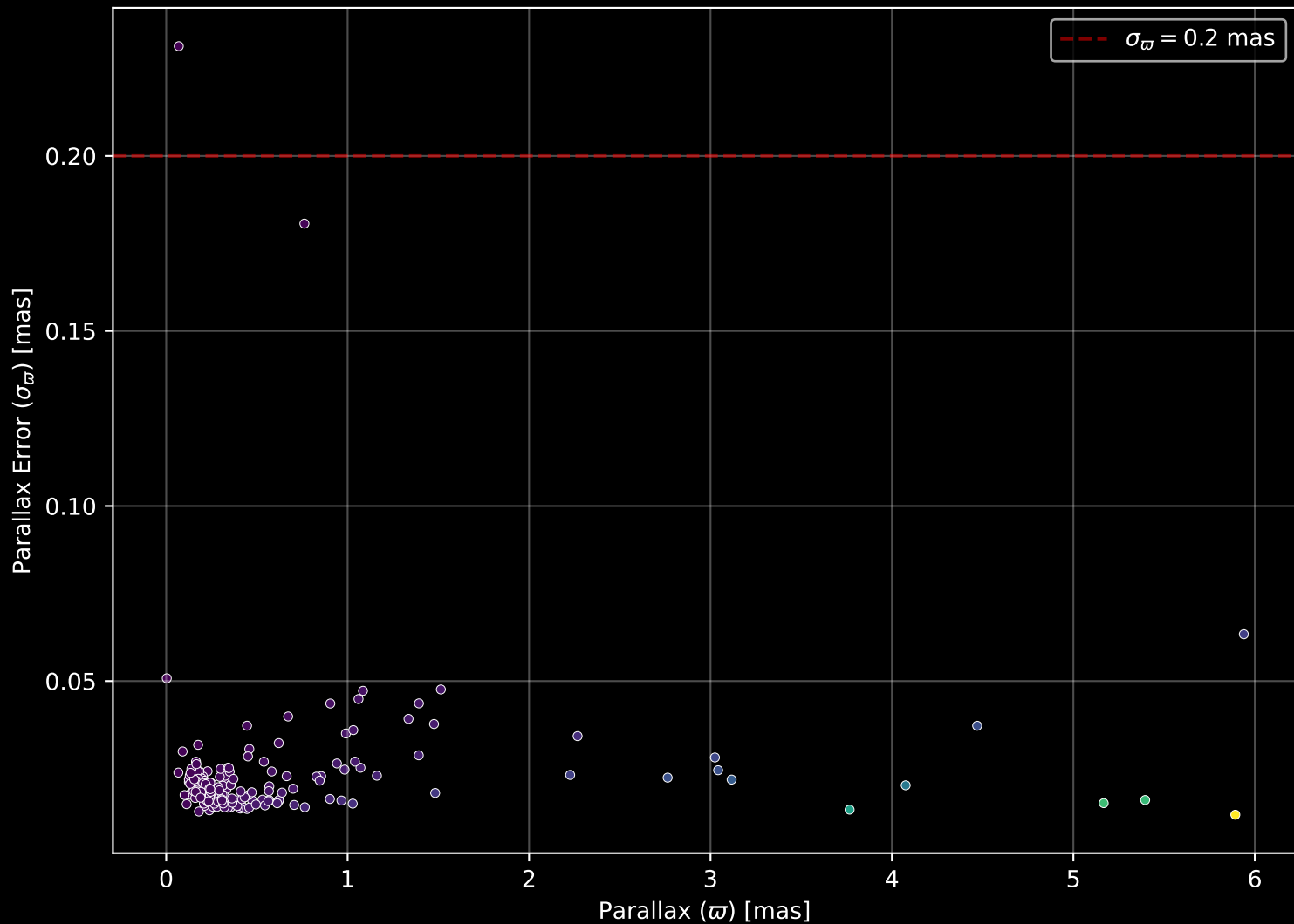
APOGEE DR17 Field: [221+04] Parallax Quality (n= 172)
