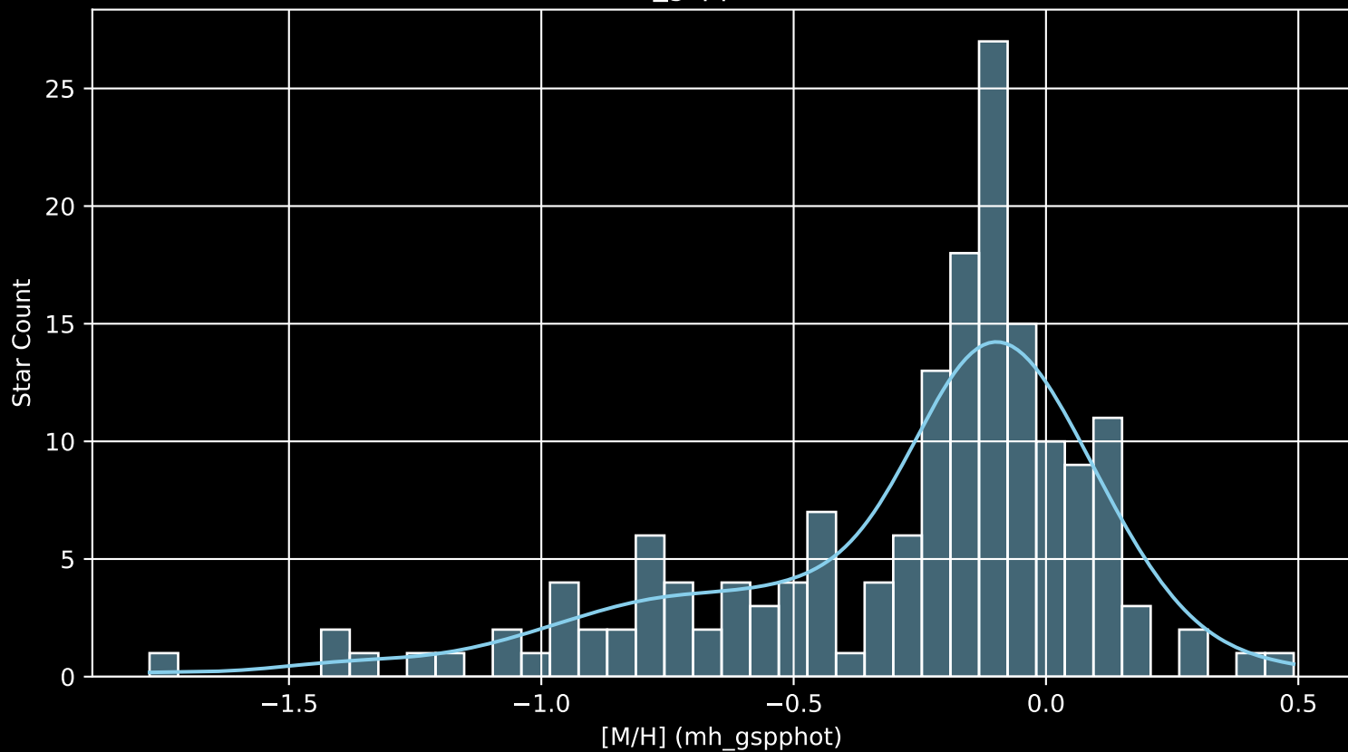
APOGEE DR17 Field: [221+04 [M/H] (mh_gspphot) (n= 168)
