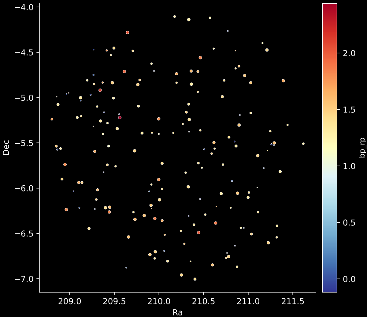
APOGEE DR17 Field: [221+04] Stars: 172
