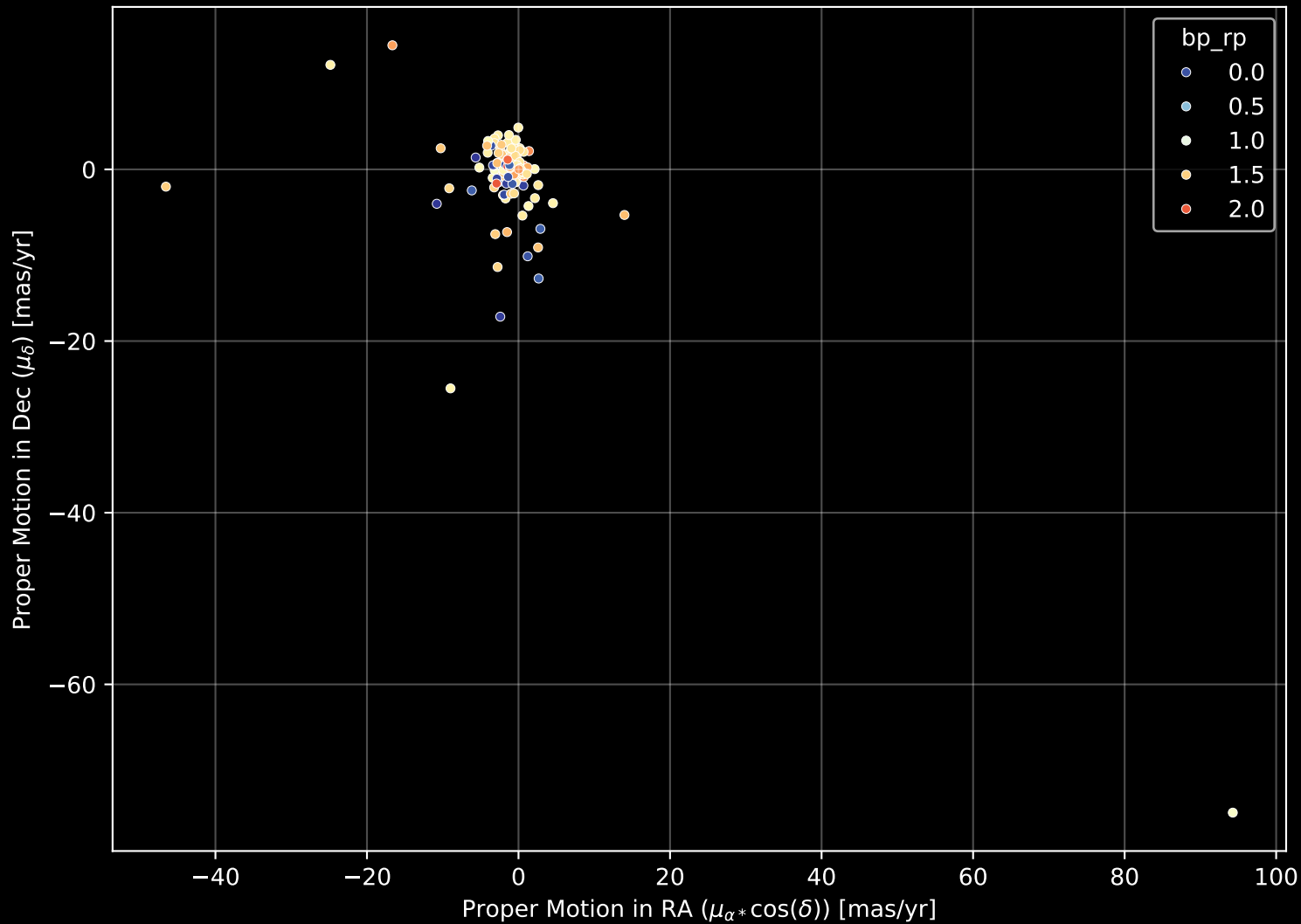
APOGEE DR17 Field: [221+04] Proper Motion Diagram (n= 172)
