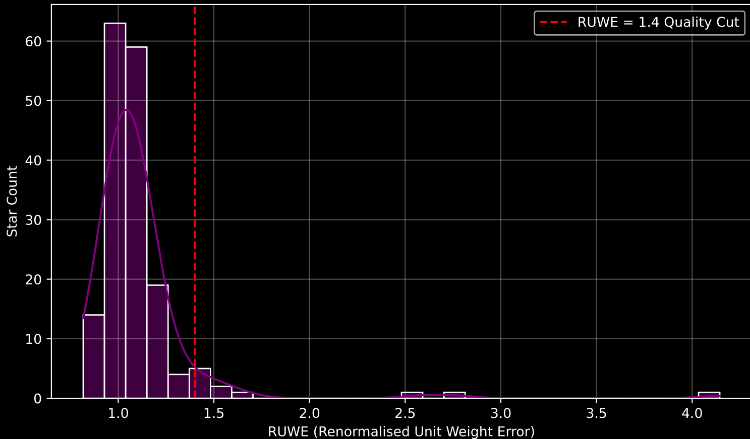
GAPOGEE DR17 Field [221+04] RUWE Distribution (n= 170)
